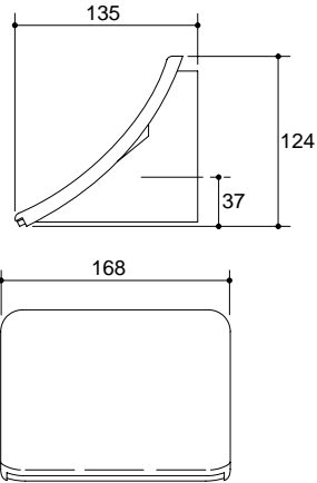
Sheetflow Bath Spout K-6946-CP
