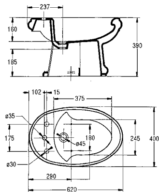
Revival Bidette D-1K83/3K83
