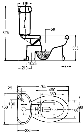
Revival Toilet D-7K93/8K94
