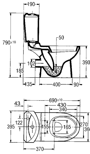
Odeon P-Trap Toilet D-OK55
