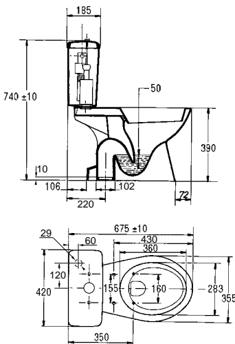
Brive® Toilet D-21073/21967
