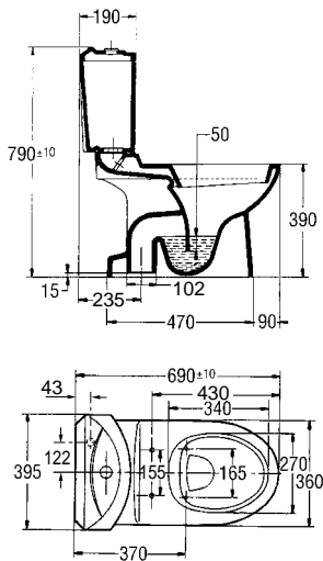
Odeon S-Trap Toilet D-OK61
