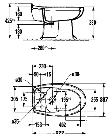
Portrait Bidette D-1790/91
