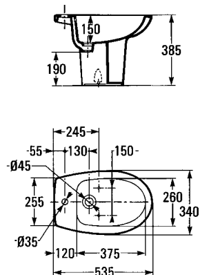
Brive Bidette D-1K88
