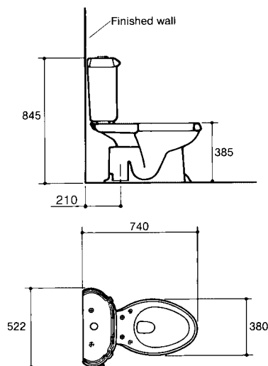
Portrait® Toilet D-1653/54
