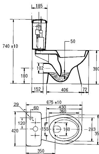
Brive P-Trap Toilet D-21072/21967
